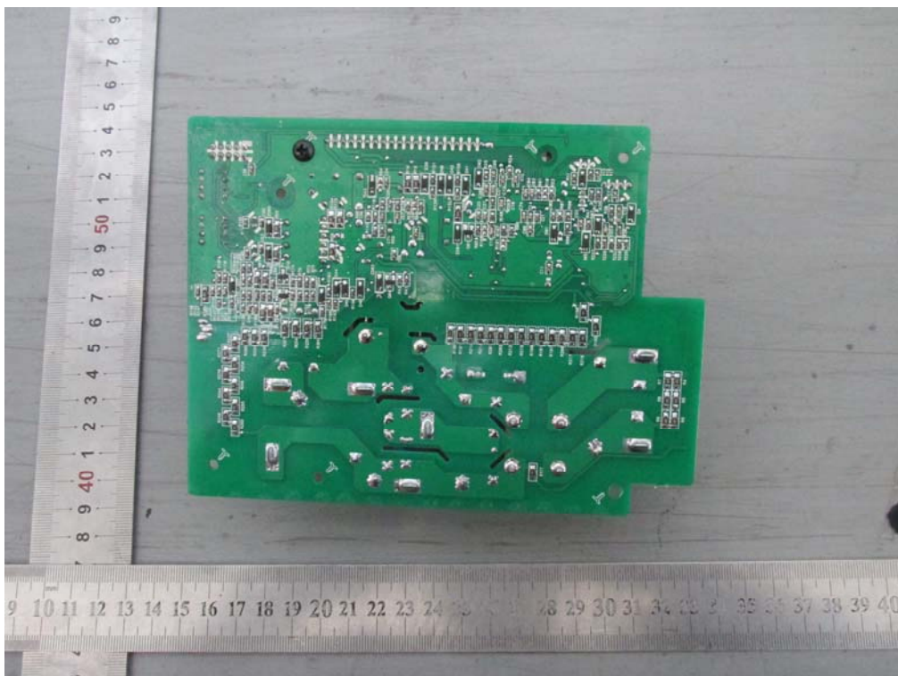
Fig. 7 –Power board view
