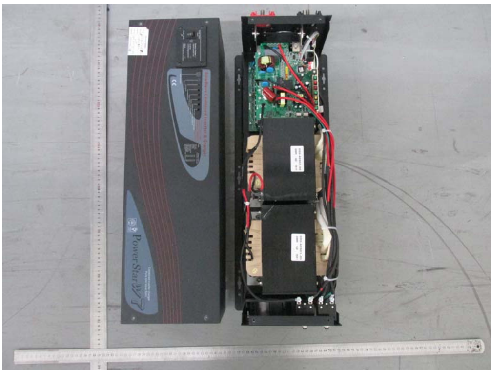
Fig. 5 –Inside view
